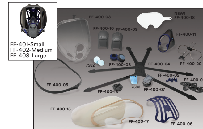
Replacement Parts For FF-400 Series Respirators FF-400-01 Buckle FF-400-02 Button FF-400-03 Lens Replacement FF-400-04 Head Harness FF-400-05 Lens Frame Assembly FF-400-06 Comfort Cradle FF-400-07 Exhalation Valve Assembly FF-400-08 Bayonet Assembly FF-400-09 Exhalation Valve Cover FF-400-10 Solid Exhalation Valve Cover FF-400-11 Nose Cup Assembly FF-400-13 Speaking Diaphragm Assembly FF-400-15 Lens Cover FF-400-17 Semi-permanent Lens Protector FF-400-18 Stacked Lens Cover 7 Layers (NEW) 7582 Inhalation Valve 7583 Exhalation Valve
