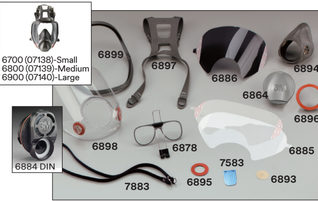
Replacement Parts For 6000 Series Full Facepiece Respirators 6878 (07141) Spectacle Kit 6880 (not shown) Cap 6884 DIN 6885 (07142) Face Shield Covers 6886 Tinted Lens Cover 7583 Exhalation Valve 6884 (37000) Center Adapter Assembly 6893 (07144) Inhalation Valve 6894 (37004) Nose Cup 6895 (07145) Inhalation Gasket 6896 Adapter Gasket 6897 (37005) Head Harness Assembly 6898 (37006) Lens Assembly 6899 (37007) Frame Kit 7883 Neck Strap
