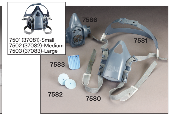
Replacement Parts For 7500 Series Half Facepiece Respirators 7580 Replacement Strap 7581 Head Harness Assembly 7582 Inhalation Valve 7583 Exhalation Valve 7586 Cartridge/Filter Holder (includes valves, not shown)
