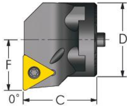
Positive Triangle (0° Lead) Coolant Thru
