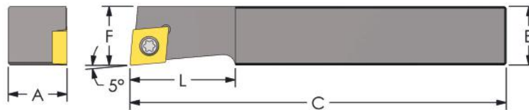
Positive 80° Diamond (-5° Lead)
